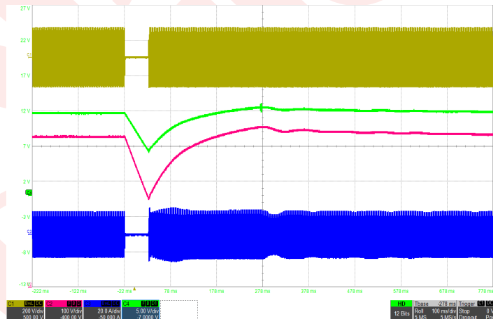
Figure 10: Line drop out with 600µF hold-up capacitor at full load (115Vrms, 400Hz) Ch1: Vin (200V/div), Ch2: Vhold-up (100V/div), Ch3: Iin (20A/div), Ch4: Vout (5V/div), Timebase: (100ms/div).
