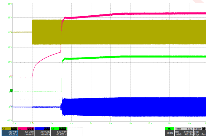
Figure 3: Typical startup waveform with 600µF hold-up capacitor (115Vrms, 60Hz) Ch1: V_{in} (200V/div), Ch2: Hold-up capacitor voltage (100V/div), Ch3: I_{in} (20A/div), Ch4: V_{out} (5V/div), Timebase: (2s/div).
