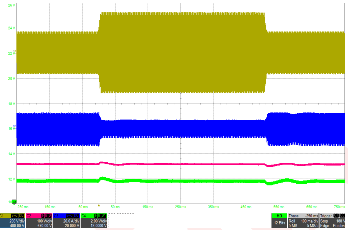
Figure 8: Input transient with 600µF hold-up capacitor at full load (115Vrms-220Vrms-115Vrms, 400Hz) Ch1: Vin (200V/div), Ch2: Vhold-up (100V/div), Ch3: Iin (20A/div), Ch4: Vout (2V/div), Timebase: (100ms/div).
