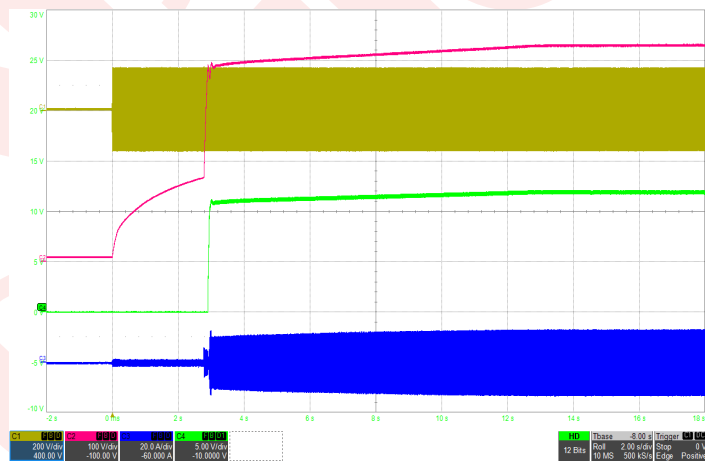
Figure 4: Typical startup waveform with 600µF hold-up capacitor (115Vrms, 400Hz) Ch1: V_{in} (200V/div), Ch2: Hold-up capacitor voltage (100V/div), Ch3: I_{in} (20A/div), Ch4: V_{out} (5V/div), Timebase: (2s/div).
