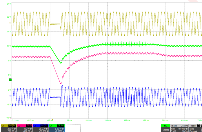
Figure 9: Line drop out with 600µF hold-up capacitor at full load (115Vrms, 60Hz) Ch1: Vin (200V/div), Ch2: Vhold-up (100V/div), Ch3: Iin (20A/div), Ch4: Vout (5V/div), Timebase: (100ms/div).
