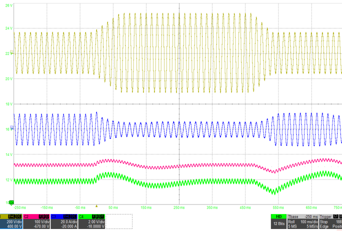
Figure 7: Input transient with 600µF hold-up capacitor at full load (115Vrms-220Vrms-115Vrms, 60Hz) Ch1: Vin (200V/div), Ch2: Vhold-up (100V/div), Ch3: Iin (20A/div), Ch4: Vout (2V/div), Timebase: (100ms/div).
